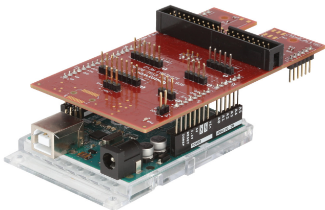
Figure 2. SEB Arduino Assembly
